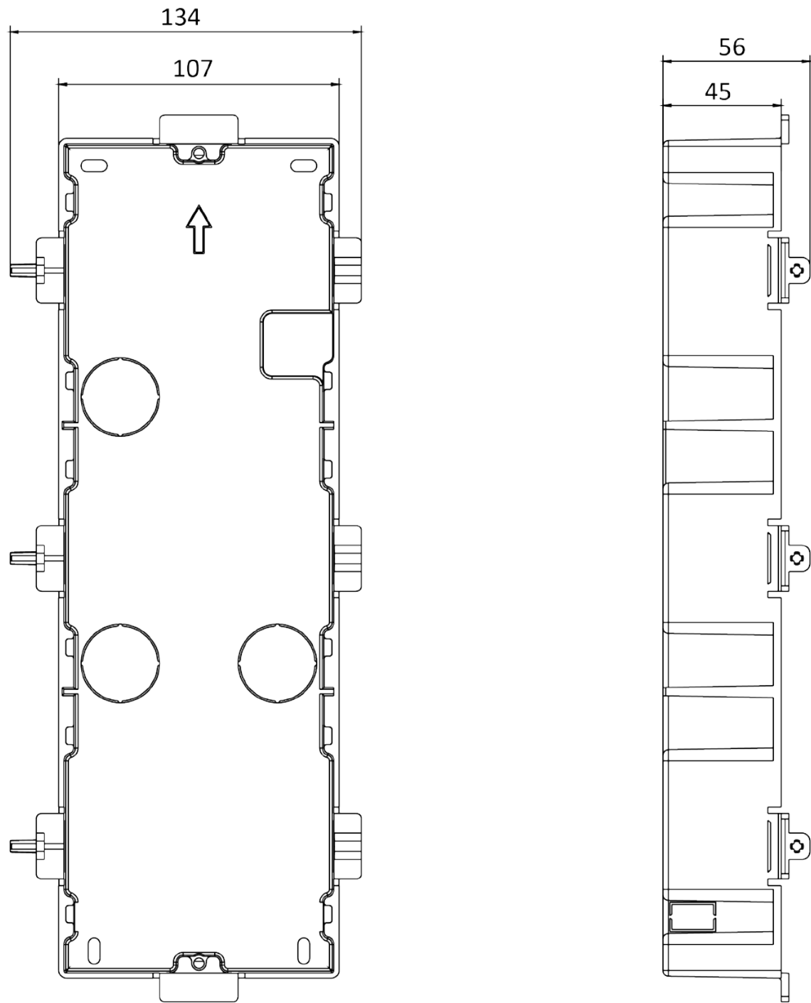
Figure 4-36 Gang Box
