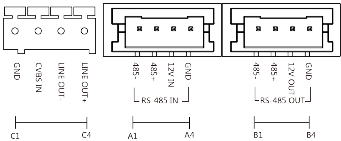
Figure 3-4 Touch-Display Module
