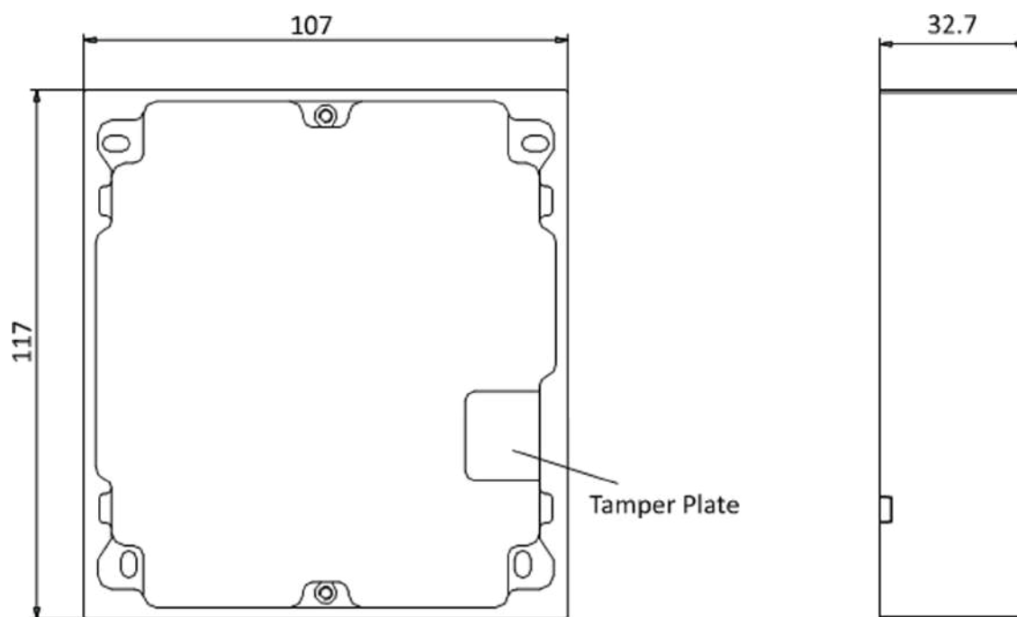
Figure 4-1 Mounting Frame
